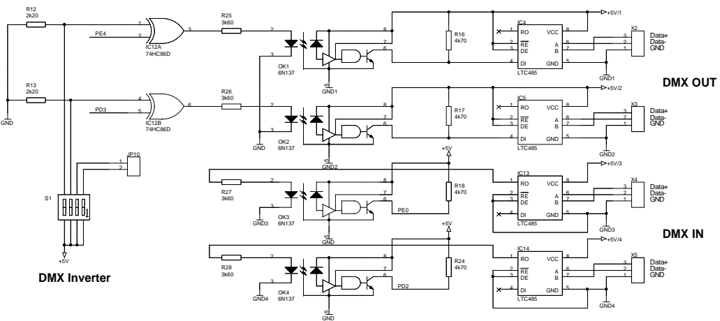
DMX Inverter
