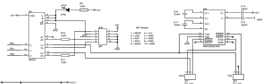
DMX OUT
